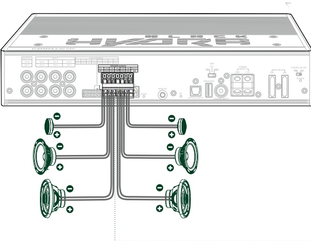
Example 2. Speakers outputs: 2-way front + broadband rear.
