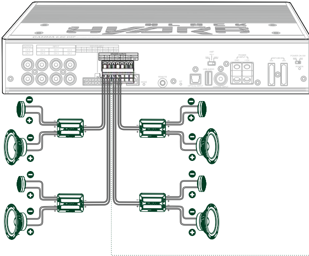
Example 1. Speakers outputs: 2-way front + 2-way rear.
