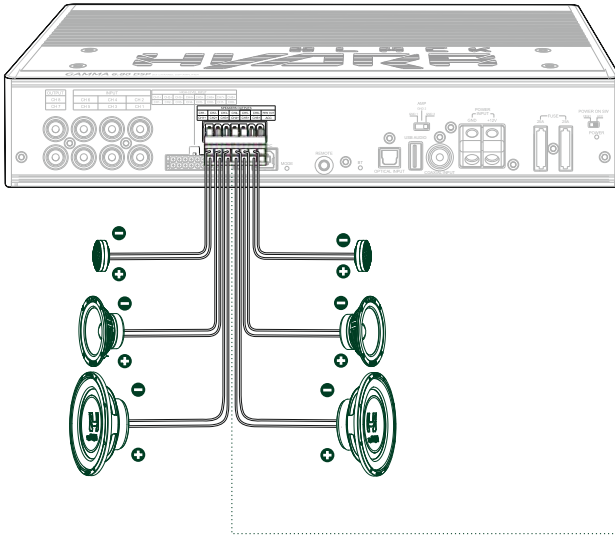
Example 3. Speakers outputs: 2-way front + two subwoofers
